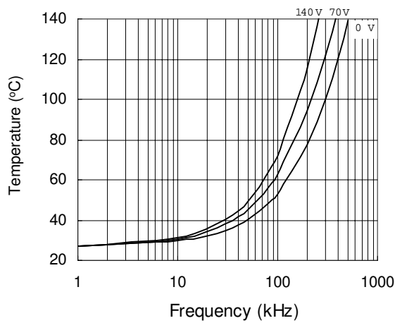
Figure 39. IRS21064S vs. Frequency (IRFPE50), R_{gate}=10 \Omega , V_{CC}=15 \text{ V}
