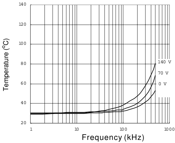
Figure 37. IRS21064S vs. Frequency (IRFBC30), R_{gate}=22 \Omega , V_{CC}=15 \text{ V}
