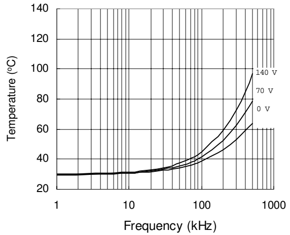
Figure 38. IRS21064S vs. Frequency (IRFBC40), R_{gate}=15 \Omega , V_{CC}=15 \text{ V}
